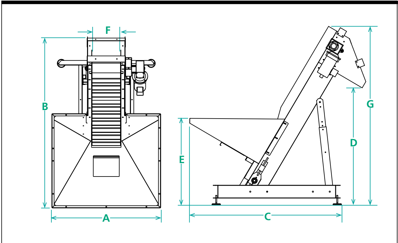
Figure 1-4. EP-10/20/30 Dimension Views
