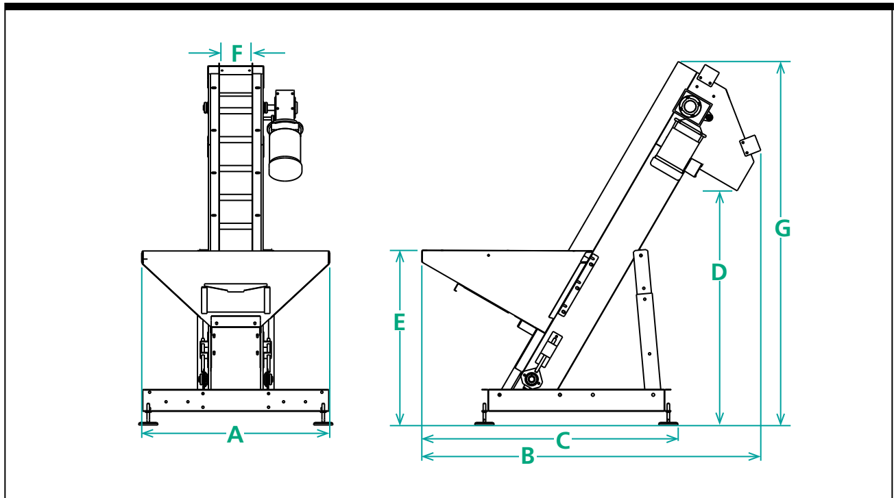
Figure 1-2. EP-04/06 Dimension Views
