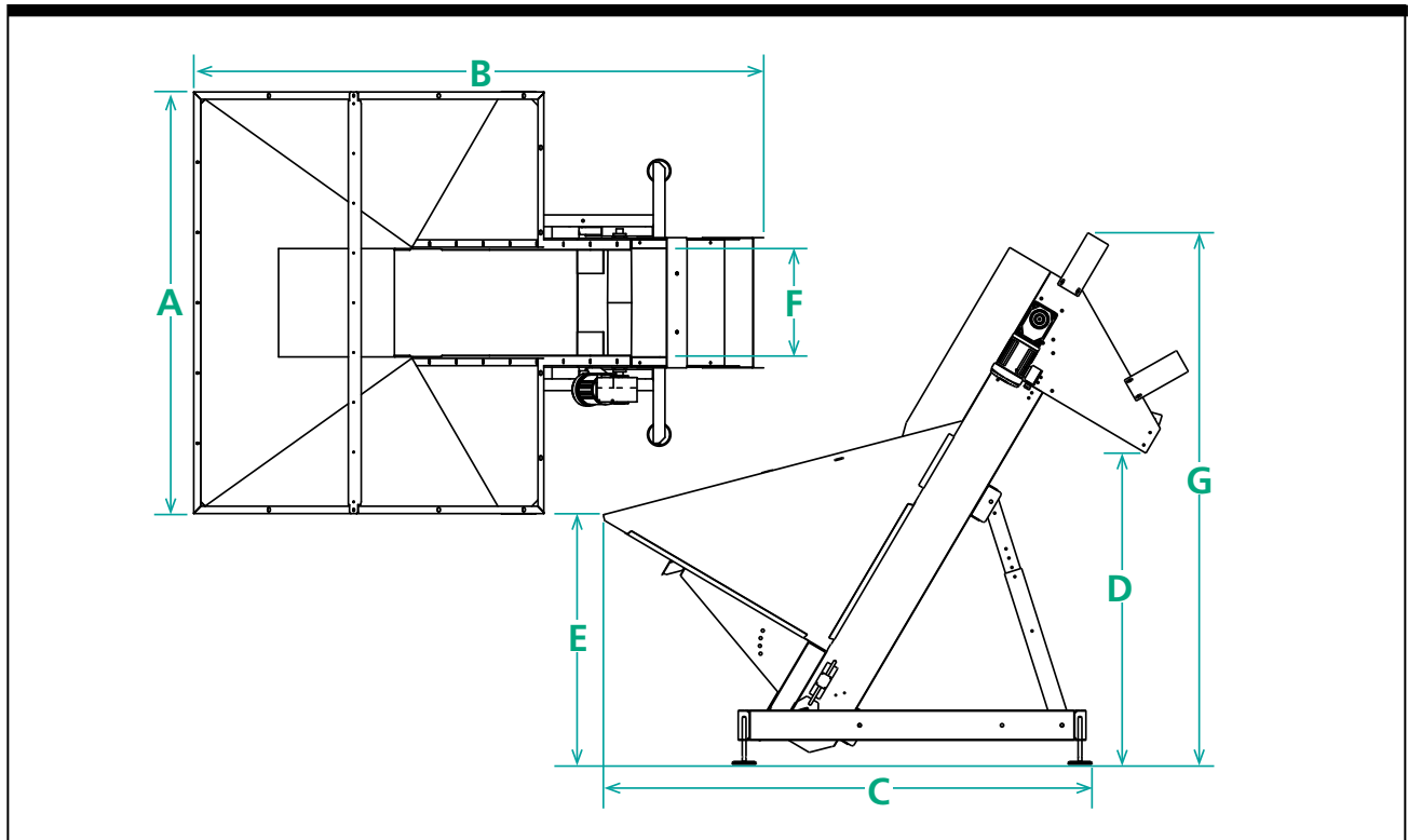
Figure 1-5. EP-35/50 Dimension Views Views
