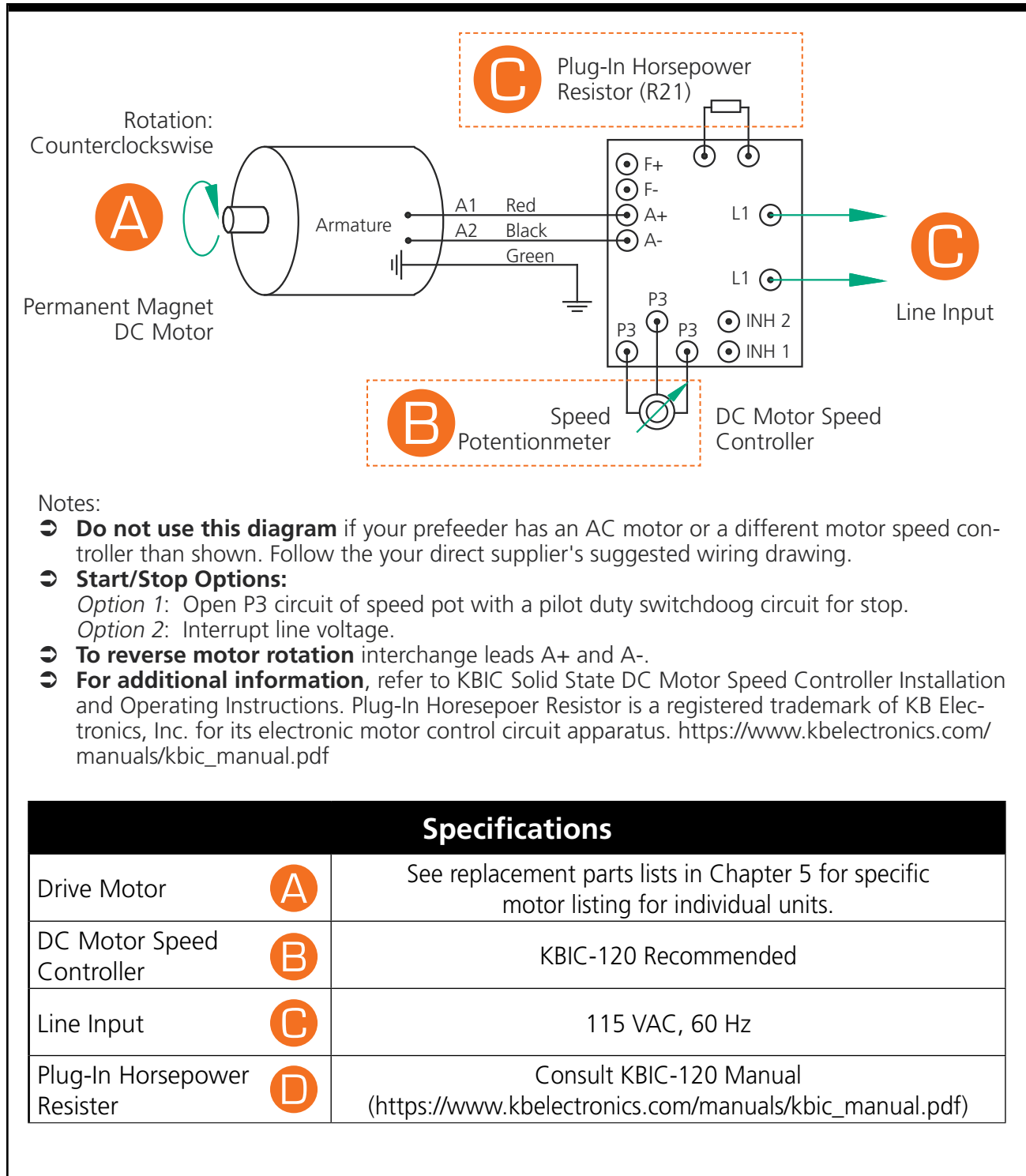
Figure 3-14. Wiring Diagram - DC Prefeeder
