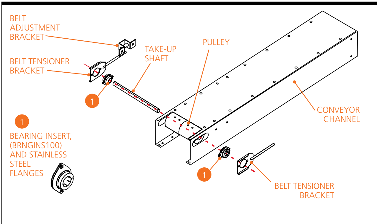
Figure 4-2. Lower Take-Up Pulley Sub-Assembly
