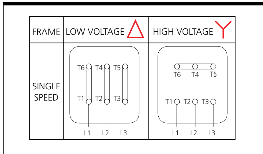
Figure 3-13. Wiring Diagram - AC Prefeeder
