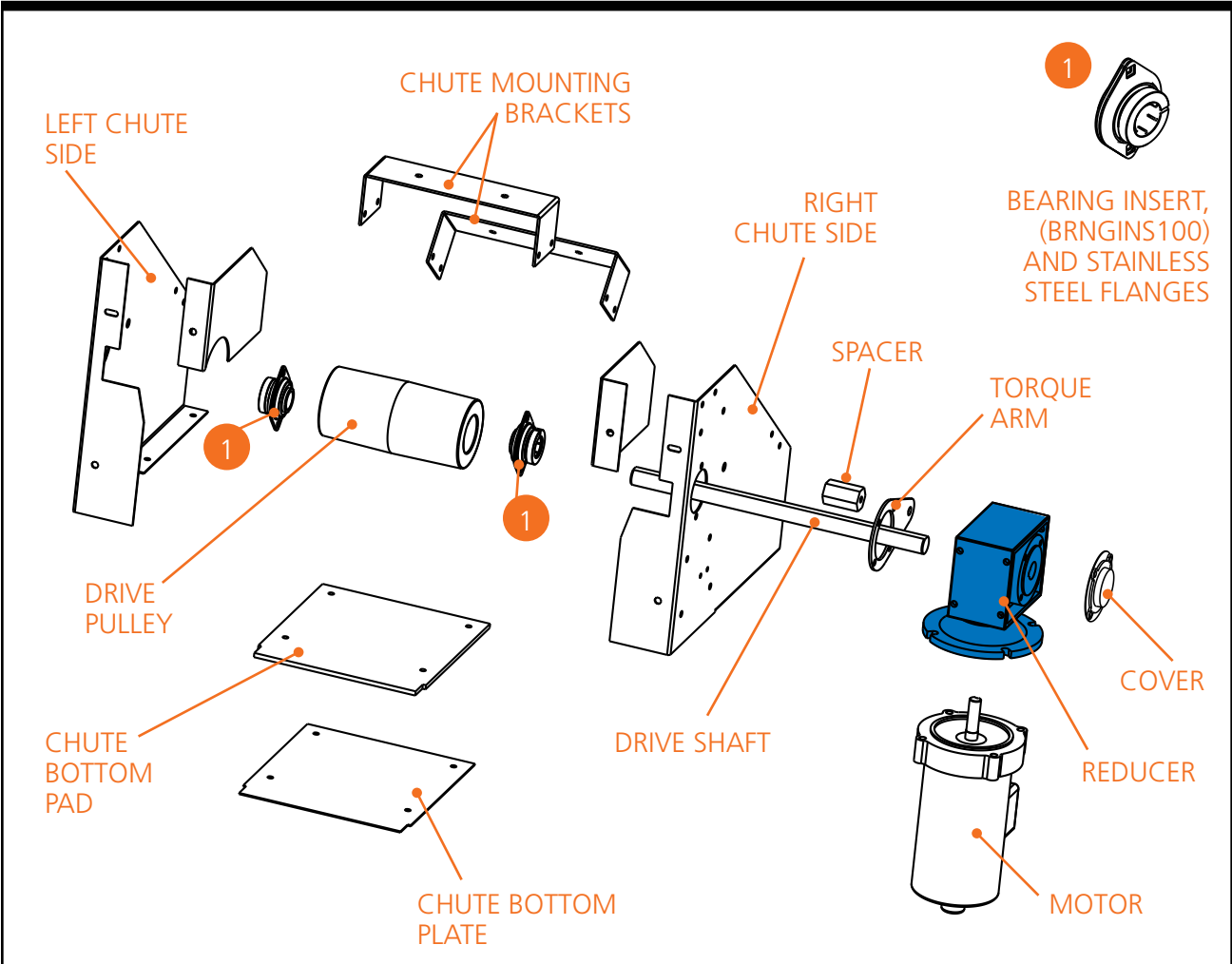
Figure 4-1. Drive Pulley (Head) with Motor/Reducer Sub-Assembly (DC Motor Shown)
