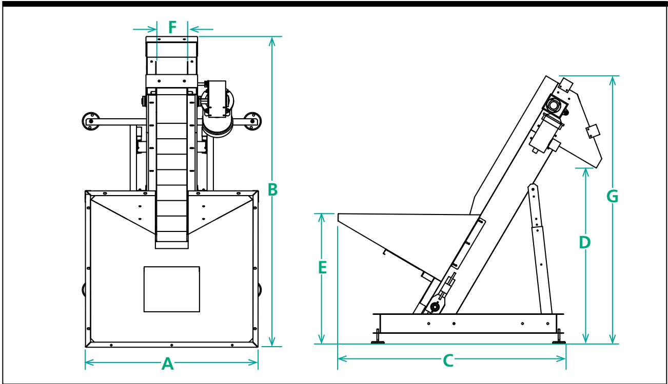
Figure 1-3. EP-08/15/25 Dimension Views
